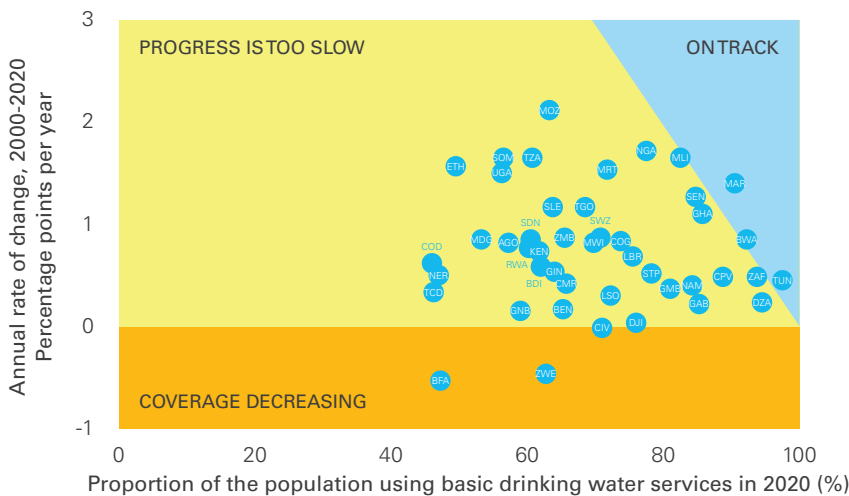
Figure 4: Progress towards universal access to at least basic drinking water services (2000-2020) among countries with <99% national coverage in 2020
